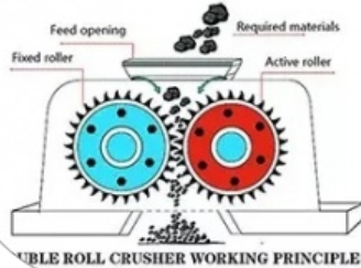
ROLLER CRUSHER WORKING PRINCIPLE
