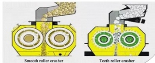
Smooth roller crusher
